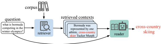
(a) Retrieval-Augmented Approach
