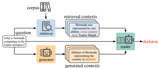
(c) Hybrid Approach
